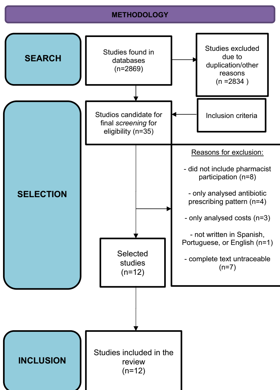
Fig. 1. Selection of studies.
